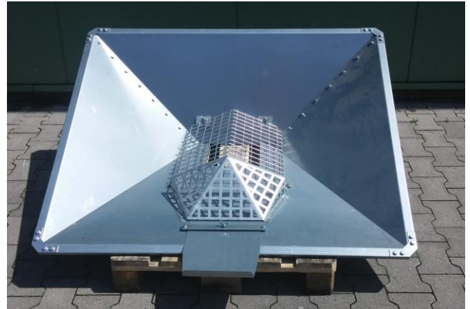
Trichter RGK 1,36x1,16m
